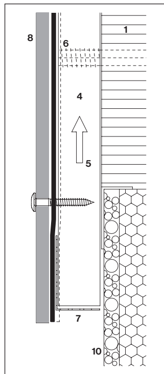
Timber verticals with spacer screw
