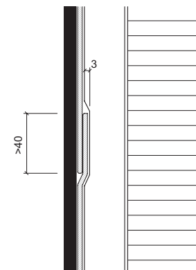
EPDM strip overlap
